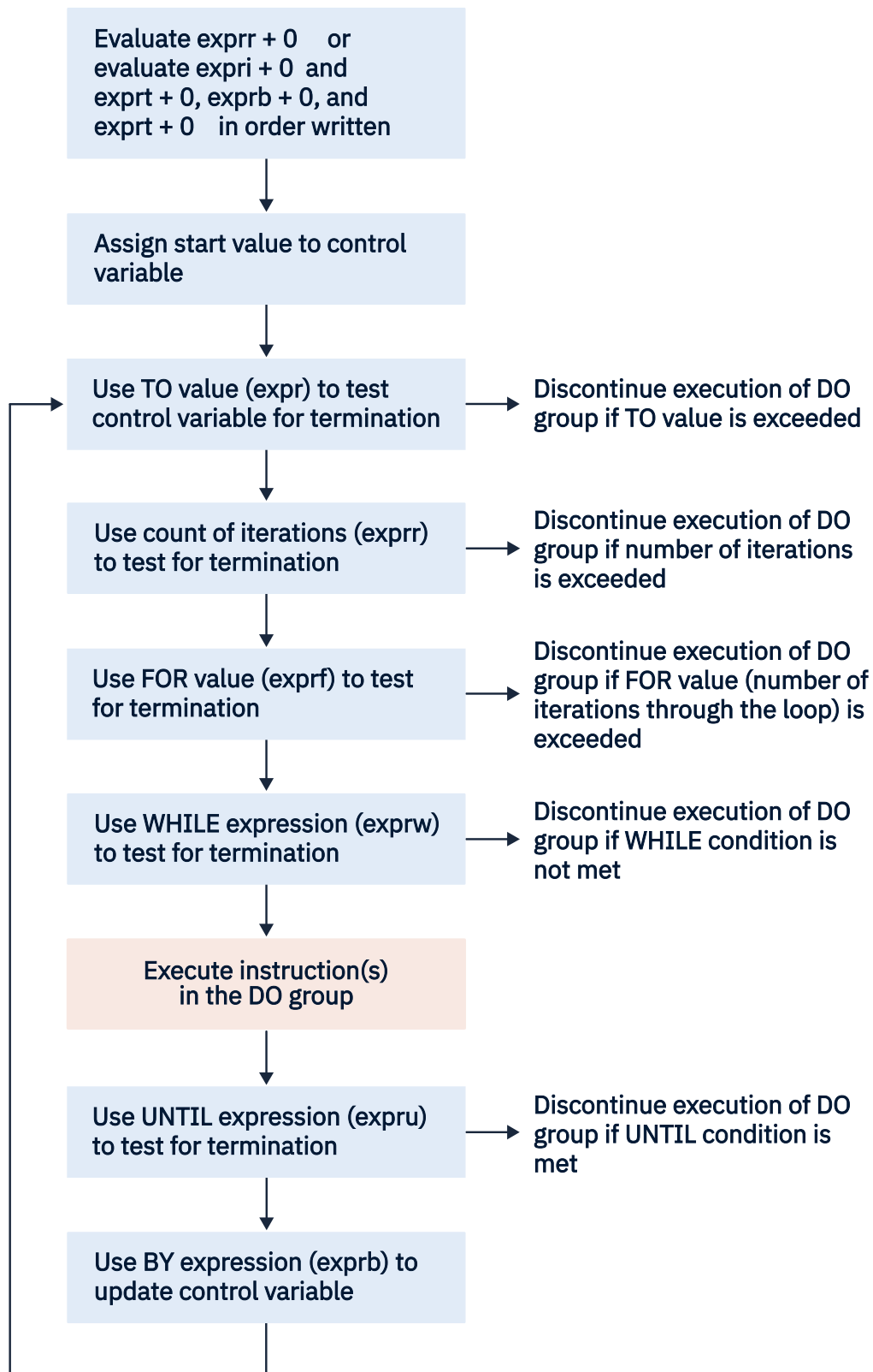
Figure 46. Concept of a DO Loop
