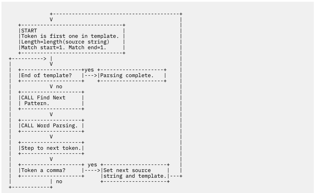
Figure 47. Conceptual Overview of Parsing
