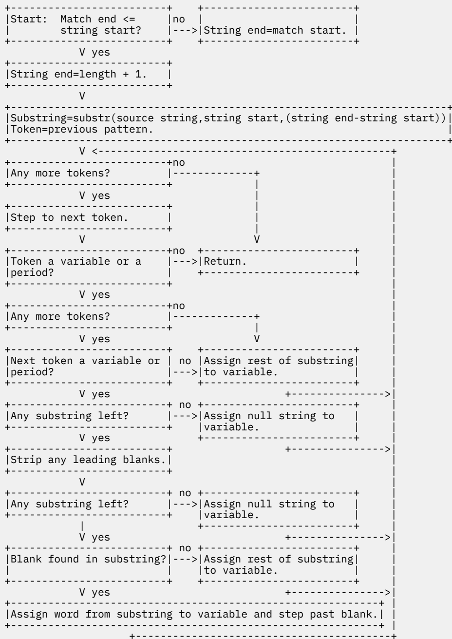
Figure 49. Conceptual View of Word Parsing
